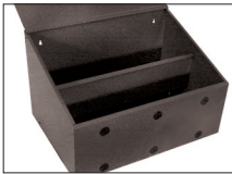
FUEL / VACUUM LINE DISPENSER F03131 • An easy to use dispenser for fuel and vacuum hoses • Holds reels up to 6-1/2" in diameter • Grommets on front hold hose in place, ready for dispensing • Hinged top helps keep hoses clean • Dimensions: 12" H x 19-1/2" W x 14" D Nominal • Designed to be able to be placed on top of a 4-drawer rack system • Ruler is painted on lid for easy measuring of hose lengths
